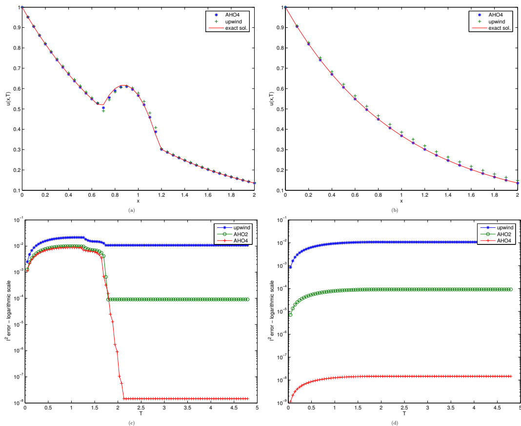
FIGURE 1. Linear hyperbolic example, subsection (7.1). In figure (a) and (b) we plot the solution to the upwind scheme (7.4) and to the AHO4 scheme (3.16) for problem (7.2)-(7.7) coupled with the exact solution (7.3). In (a) we show that after few time iterations the initial perturbation is still dominant and the schemes have the same accuracy, while in (b), increasing time, the initial perturbation vanishes and the numerical solution using upwind loses the steady state while using AHO4 not. To make this more clear, in figure (c) we fix h = 0.05 and we compare the l^2 -error (7.1) using upwind, AHO2, AHO4 schemes, increasing time. Then, it is evident that, once the steady state has been reached, the AHO2-error ( \circ ) decays rapidly to its order of accuracy, as well as AHO4-error ( * ) does gaining more and more accuracy. Moreover, to confirm the order of accuracy of the AHO4 scheme, we test the three schemes upwind, AHO2, AHO4 on the steady state solution (7.6) and in figure (d) we plot the resulting errors. As we expected, we gain accuracy using the AHO4 scheme, and we can affirm that, the scheme produces no time evolution on steady state data.
