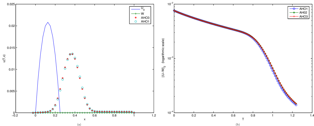
FIGURE 3. Integro-differential example, subsection (7.2). We consider schemes (7.11), (6.11), (6.12) to solve problem (7.8)-(7.13). In figure (a) we plot the three solutions coupled with the initial data (7.13), after few time iterations, when the initial perturbation is still dominant, while in figure (b) we compare the quantity (7.1) using the three schemes, for a large time simulation. Both figures (a) and (b) show that the schemes have the same accuracy. This is exactly what we expect when the initial data is a perturbation of a constant state. In fact, by consistency assumptions, all schemes should be exact when computed on constants.
