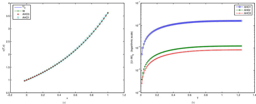
FIGURE 2. Integro-differential example, subsection (7.2). We consider schemes (7.11), (6.11), (6.12) to solve problem (7.8)-(7.12). In figure (a) we plot the solutions coupled with the steady state (7.12), while in figure (b) we compare the quantity (7.1) using the three schemes, for a large time simulation. As we expected, we gain accuracy using the AHO2 and AHO3 schemes.
