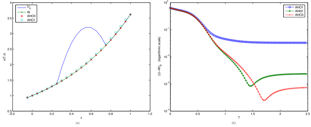
FIGURE 4. Integro-differential example, subsection (7.2). We consider schemes (7.11), (6.11), (6.12) to solve problem (7.8)-(7.14). In figure (a) we plot the solutions coupled with the initial data (7.14) after M = 100 time iterations, while in figure (b) we compare the quantity (7.1) using the three schemes, for a large time simulation. It is clear that, once the steady state has been reached, the AHO2-error (*) decays rapidly to its high-order of accuracy, as well as AHO3-error (+) does gaining more and more accuracy.
